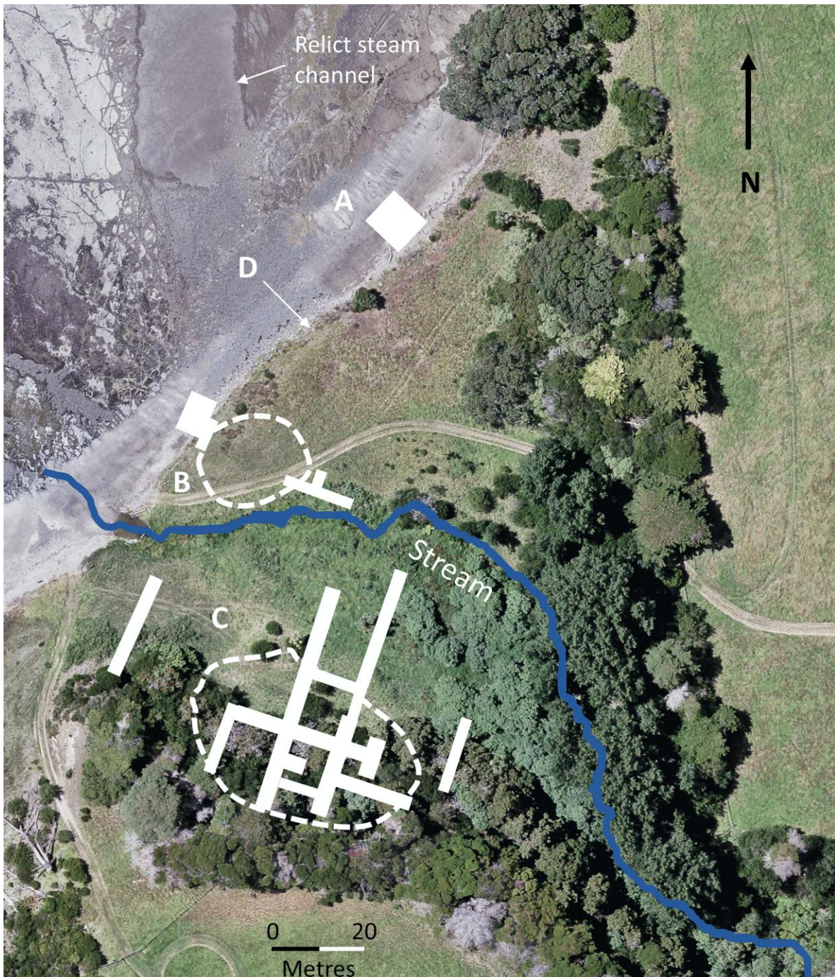
Figure 2: Pūharakeke/West Point beach (at low tide) and flat showing locations of the principal archaeological excavations and Nichol’s gravel sheet (dashed circles). A: Scott 1963; B: Nichol 1981-2 North bank of stream, including ‘oyster lens’; C: Nichol 1981-2 South bank of stream; D: Inundation deposit sample location (2009). The back-beach escarpment has retreated since the excavations of Scott and Nichol were undertaken.
